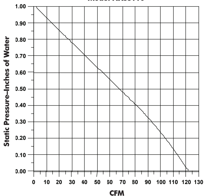
NuVent Product Performance Model NXSS110
