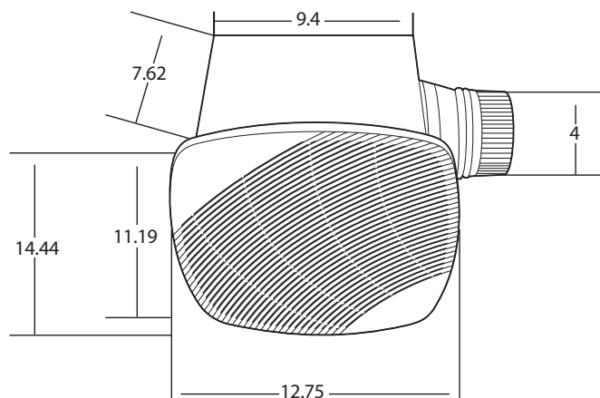
NuVent Product Performance Model NXSS110
